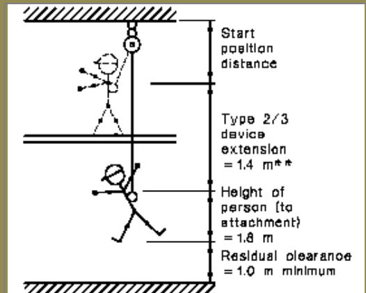
Type 2 or 3 Fall-Arrest Device
